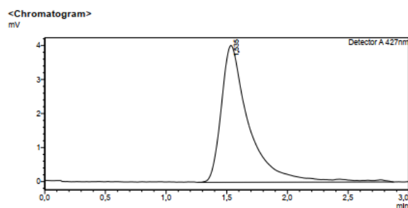
Gambar 3. Kromatogram sampel
